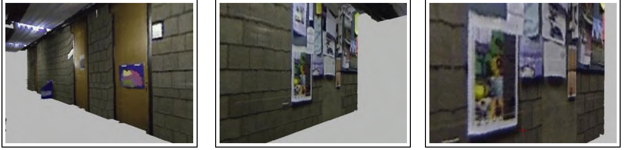
Figure 11: 3D Model generated (a) from raw sensor data, and (b) using our algorithm, in which 94.6% of all measurements are explained by 7 surfaces. Notice that the model in (b) is much smoother and appears to be more accurate.
